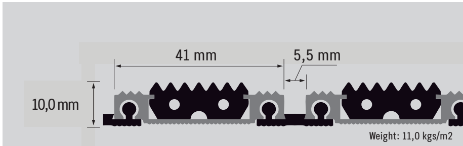
Aluminium profile
